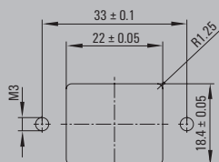
Standardised flange
