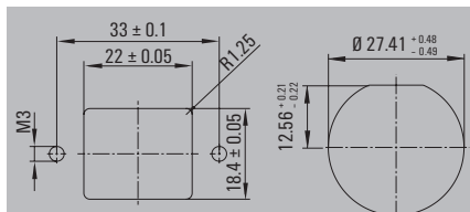
Standardised flange
