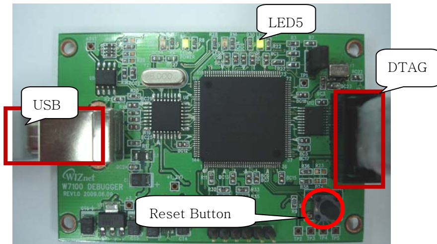
[Fig.2.2] W7100A / W7100 Debugger
