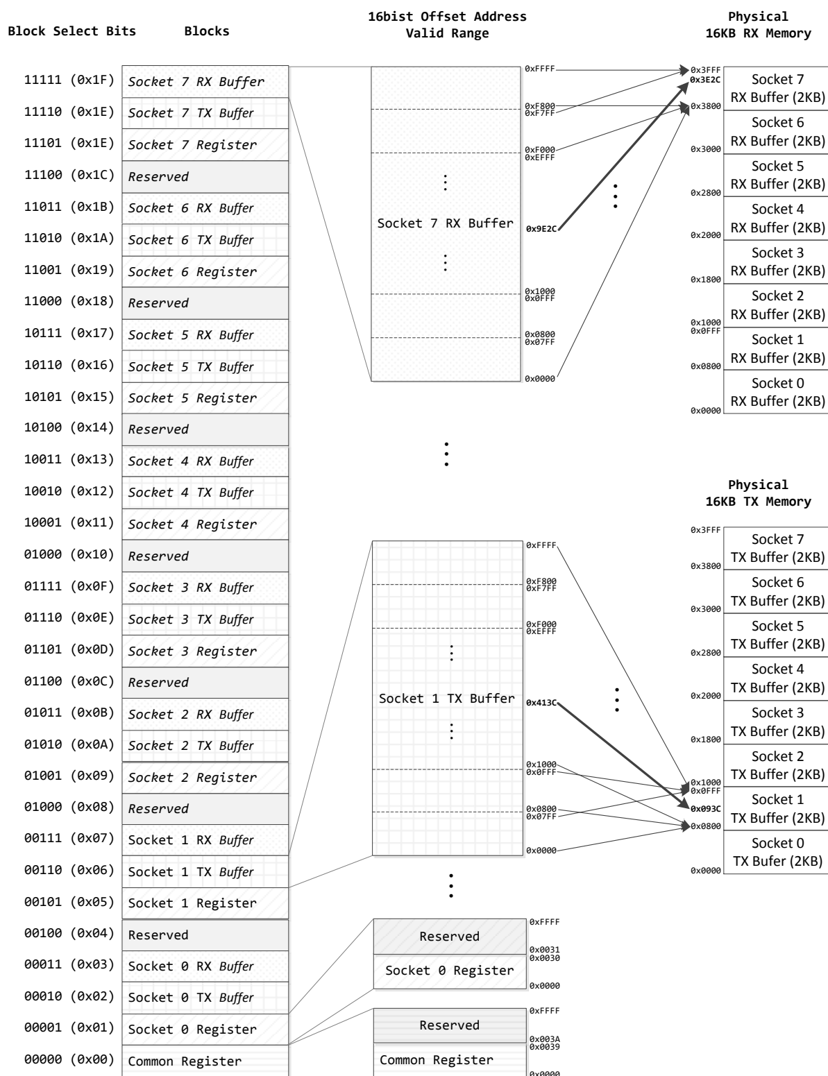
Figure 20. Register & Memory Organization
