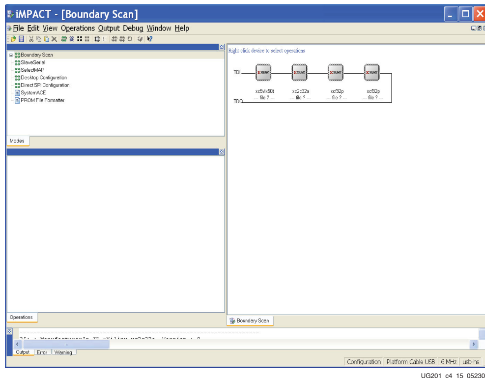
Figure 4-12: ML555 JTAG Chain with All Four Programmable Devices in the Chain
