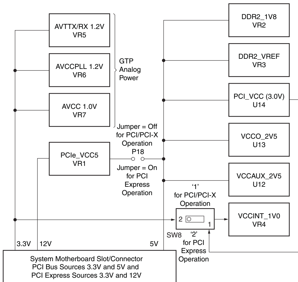
Figure 3-14: Voltage Regulator Topology
