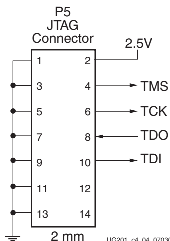
Figure 4-4: JTAG Cable Hook-up
