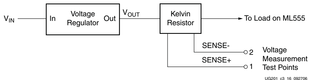
Figure 3-17: Voltage Measurement Test Points
