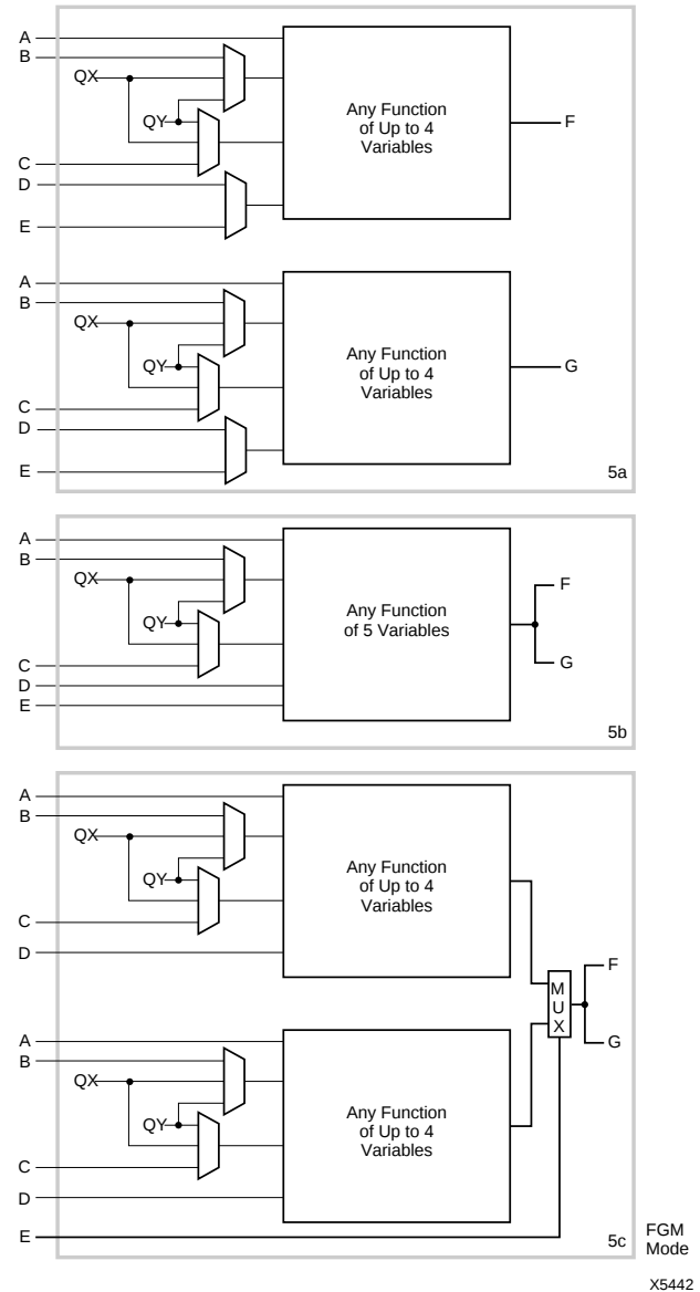
Figure 6: Combinational Logic Options
