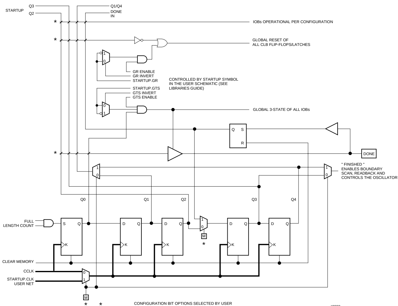
Figure 26: Start-up Logic
