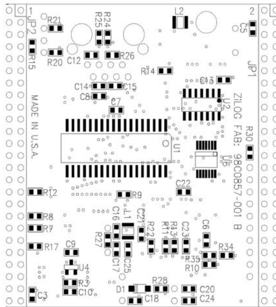
Figure 6. Bottom Layer
