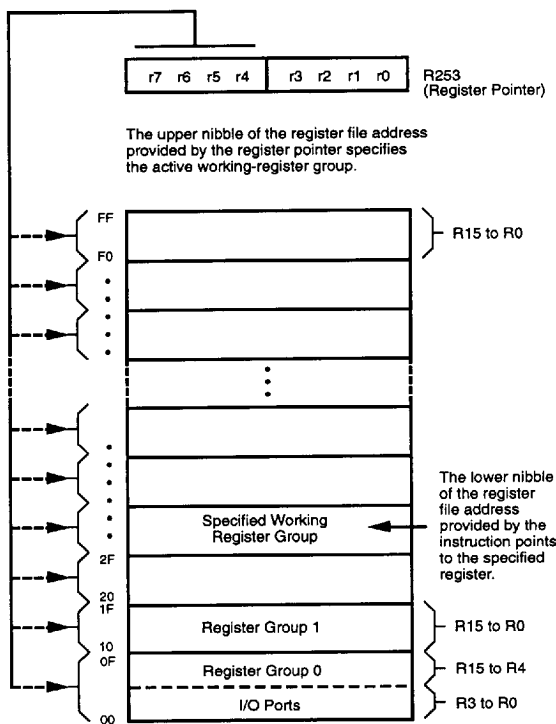
Figure 12. Register Pointer
