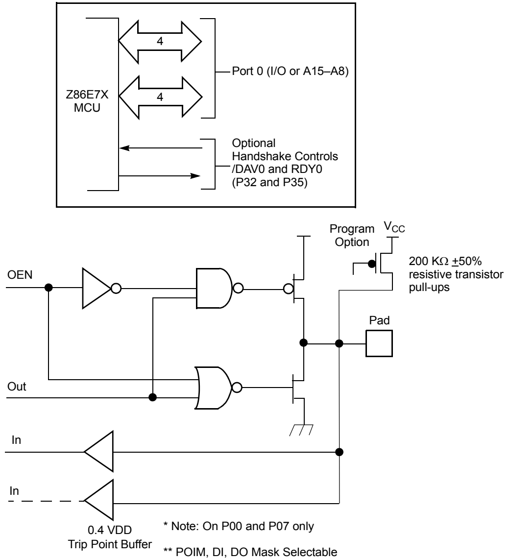
Figure 14. Port 0 Configuration
