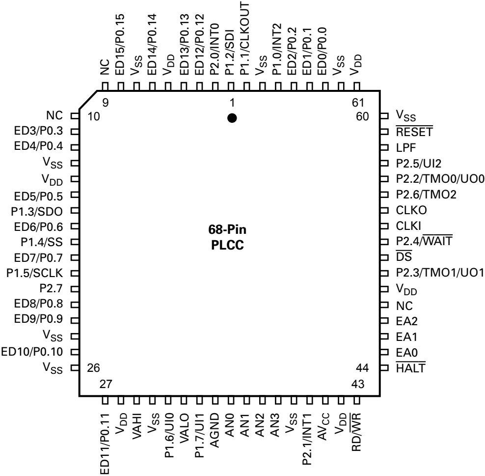
Figure 6. 68-Pin PLCC Z89323/373 Pin Configuration
