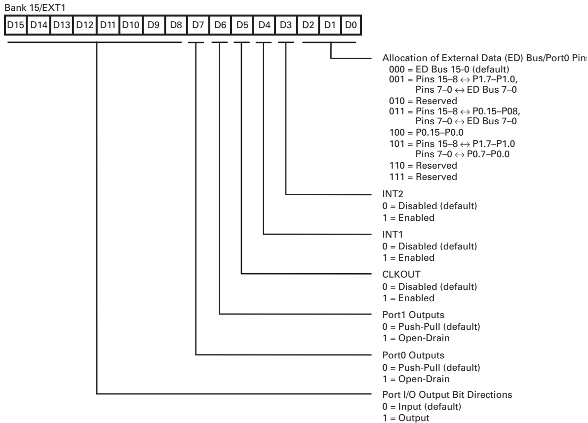
Figure 26. Bank15/EXT1 Register
