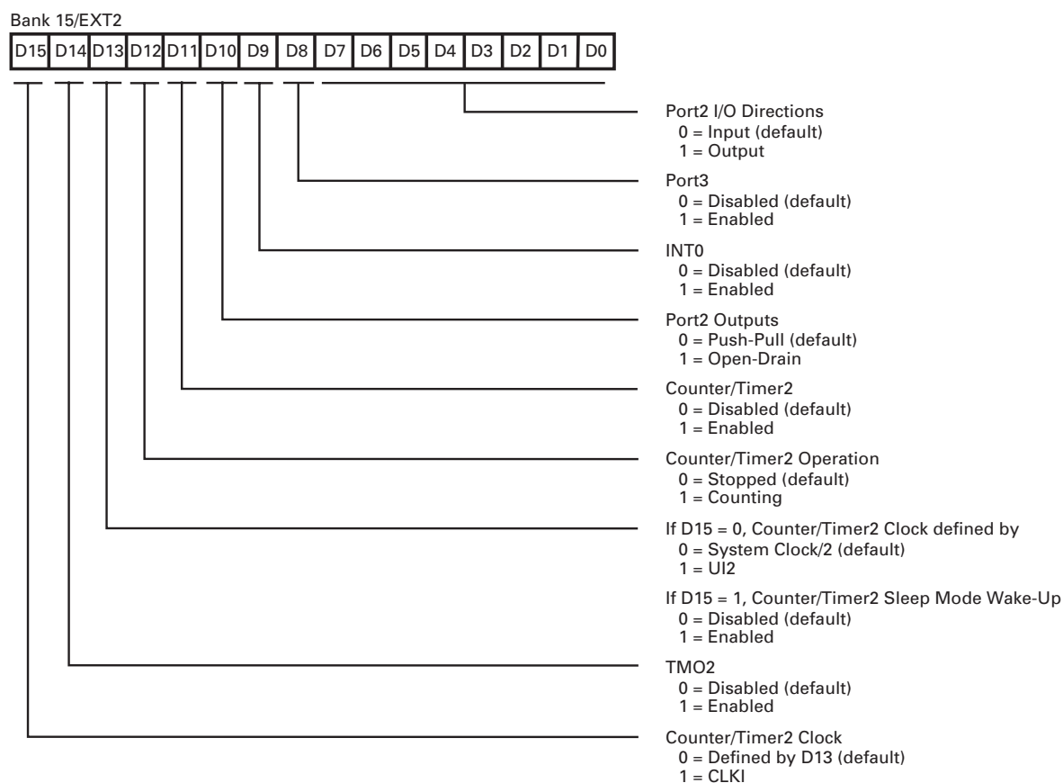
Figure 27. Bank15/EXT2 Register
