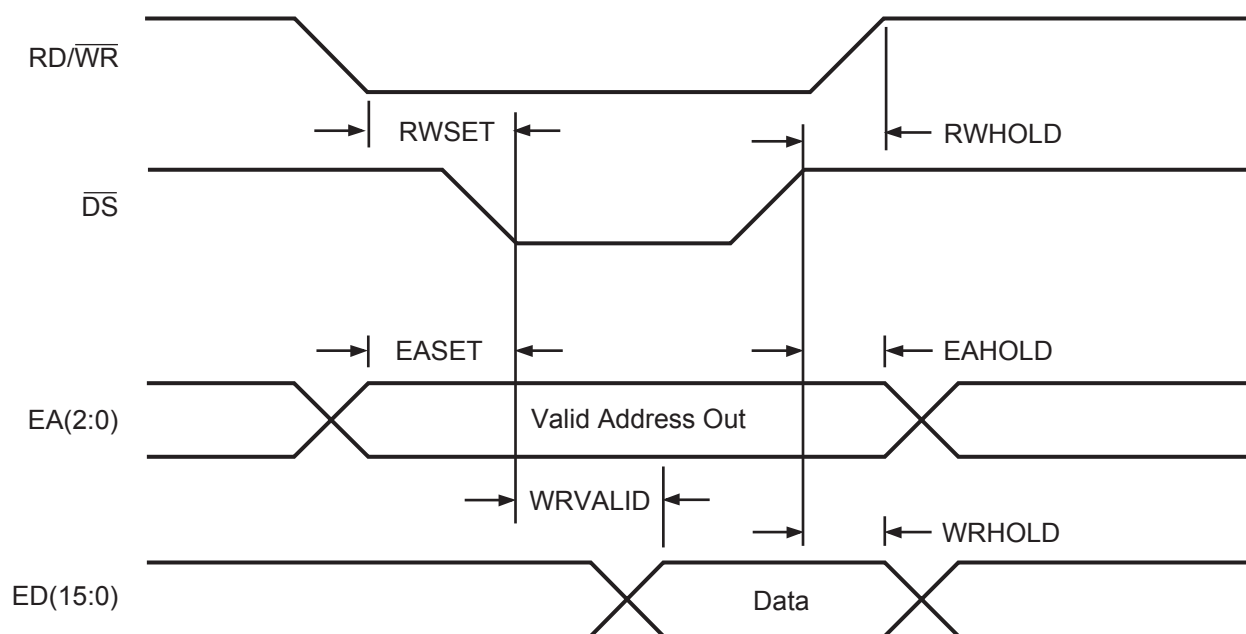
Figure 13. Write Timing
