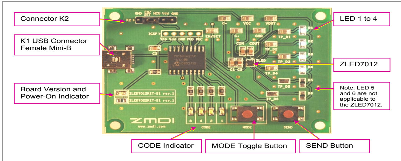
Figure 2.1 ZLED7012KIT-E1 Evaluation Board (Top View)
